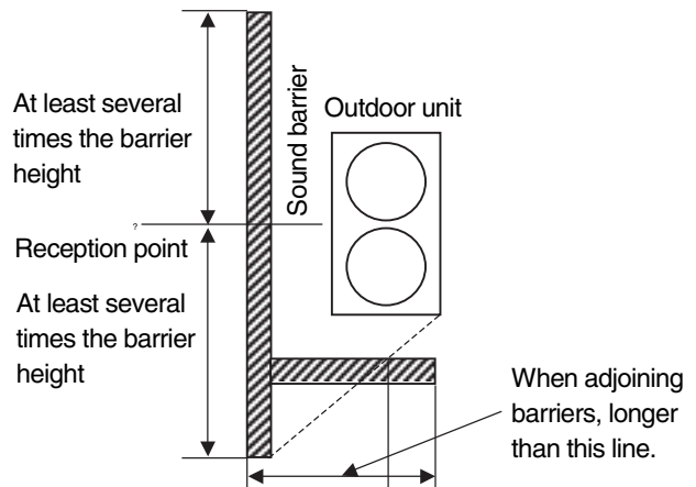
Figure 4. Sound barrier
